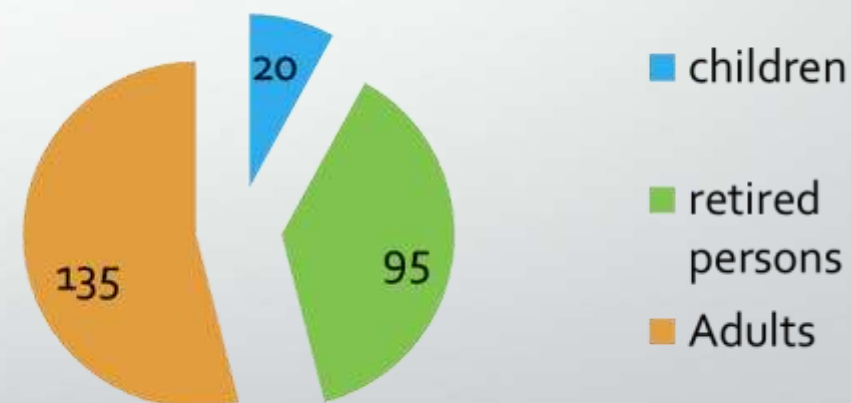
Age structure
